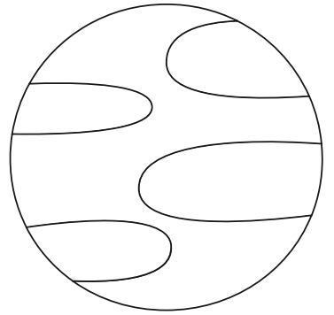
ARTIZARRA
